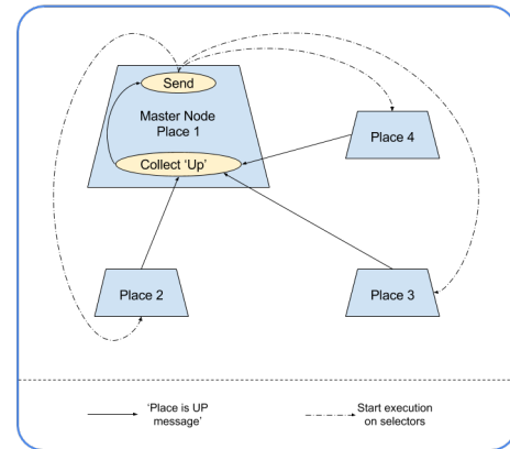
Figure 10: Bootstrap process of a distributed selector program.
