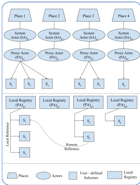
Figure 9: The Distributed Selector System
