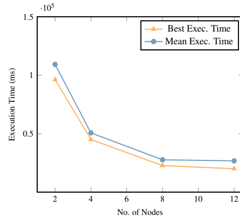
Figure 14: NQueens : Shows strong scaling of computing the NQueens problem on a 17×17 board using the described algorithm. Workers compute solutions sequentially when given a partial solution with six placed queens. The number of workers per node is constant (12). The solution limit is set to 1_477_251, which is a tenth of the size of a complete solution set. Mean Exec. time in milliseconds from 20 iterations.
