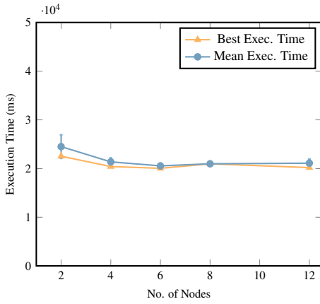
Figure 12: Trapezoidal Approximation : Shows weak scaling computing approximation with 10_000_000 pieces to calculate for each worker. Number of workers per node is constant (12), and as the number of nodes increases we increase the total number of pieces to keep the amount of work on each node constant. Mean Exec. time in milliseconds from 20 iterations.
