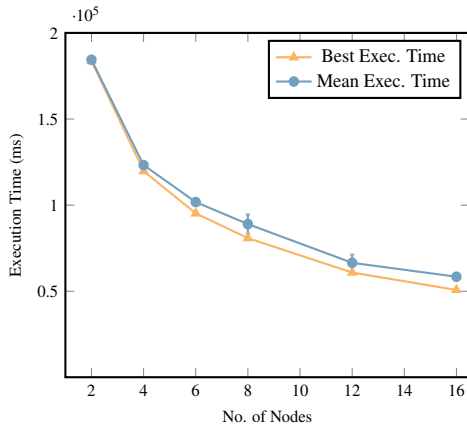
Figure 13: Precise Pi : Shows strong scaling for the calculation of Pi with a precision of 80_000. Number of workers per node is constant (12). Work is evenly distributed among all selectors. Mean Exec. time in milliseconds from 20 iterations.
