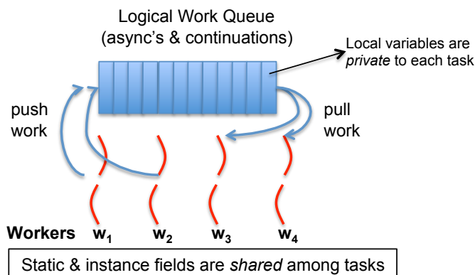
Figure 3: Scheduling a parallel program on a fixed number of workers. (Figure adapted from [9].)
