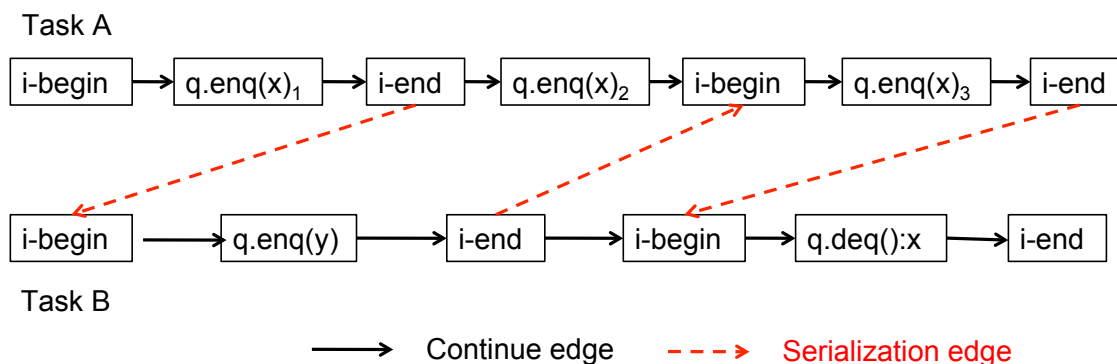
Figure 17: A Computation Graph for the execution in Table 5. q.enq(x)_1 , q.enq(x)_2 and q.enq(x)_3 refer to three steps in the q.enq(x) method, the first and third of which are enclosed in isolated statements.
