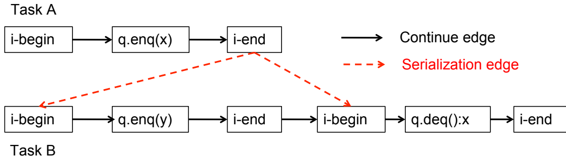
Figure 15: A Computation Graph for the execution in Table 4. i-begin and i-end refer to the beginning and end of isolated statements. q.deq():x refers to a dequeue operation that returns x .
