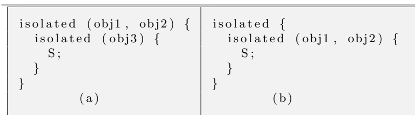
Figure 3: Simple cases for nested isolation.
