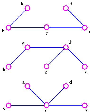
Figure 5: Three spanning trees for undirected graph in Figure 4 (source [30])
