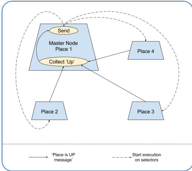
Figure 10: Bootstrap process of a distributed selector program.
