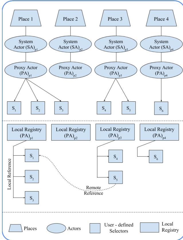
Figure 9: The Distributed Selector System
