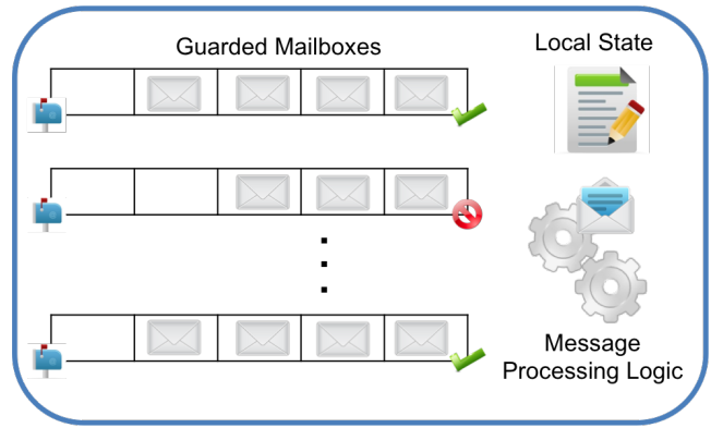
Figure 1: Decomposition of a selector: guarded mailboxes, local state, message processing logic.
