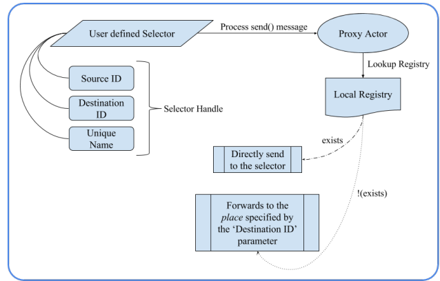
Figure 11: The Proxy Actor helps forward messages between local selectors and selectors across places .
