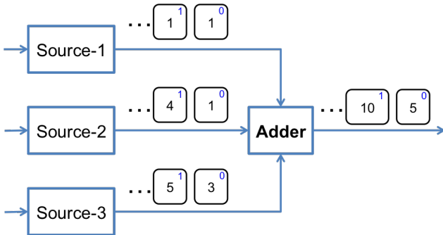
Figure 4: Actor network simulating a join pattern. Source-1, Source-2, and Source-3 are producers for data streams. The Adder actor aggregates data items from each of the three sources and sums them up.
