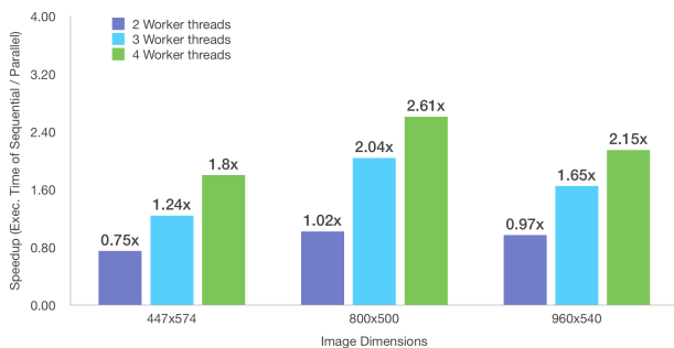
Figure 2: Speedup of the Image Filtration with different numbers of worker threads
