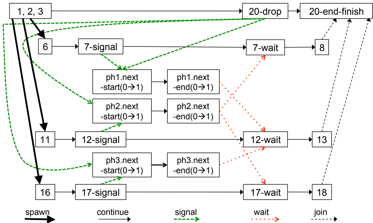
Figure 22: Computation Graph for example HJ program in Listing 36
